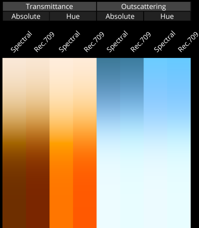
Spectral vs Rec.709 with Bruneton08 Coefficients
